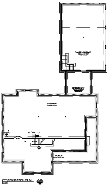
FOUNDATION PLAN
